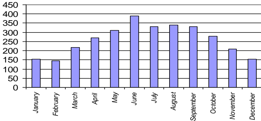
Figure (5) Evaporation measurements in the lake area in (mm)
