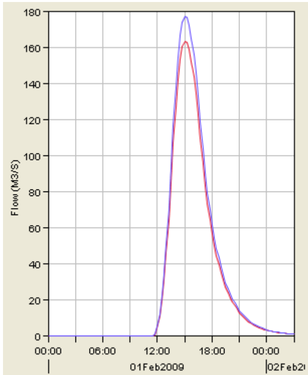
Figure (4) Runoff hydrographs for 50 and 100 year design storm
