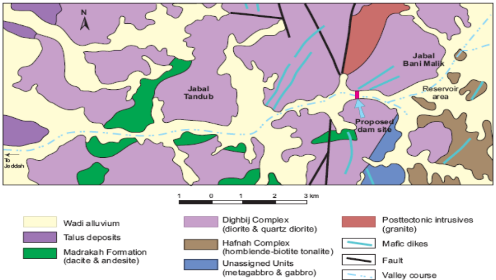
Figure (2) Geology of the study area (After Moore and Al-Rehaili, 1989)
